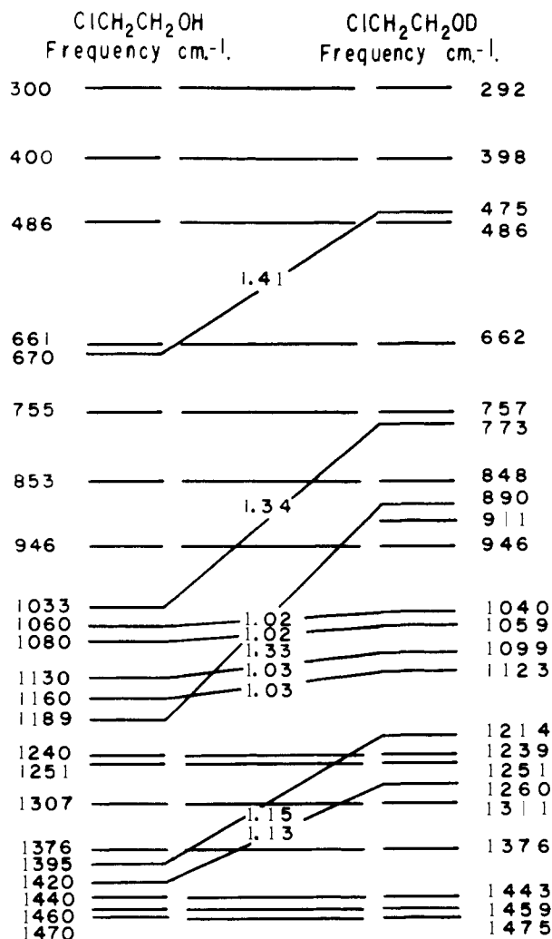
Fig. 2.—Frequency correlation diagram for 2-chloroethanol and 2-chloroethanol- d .
