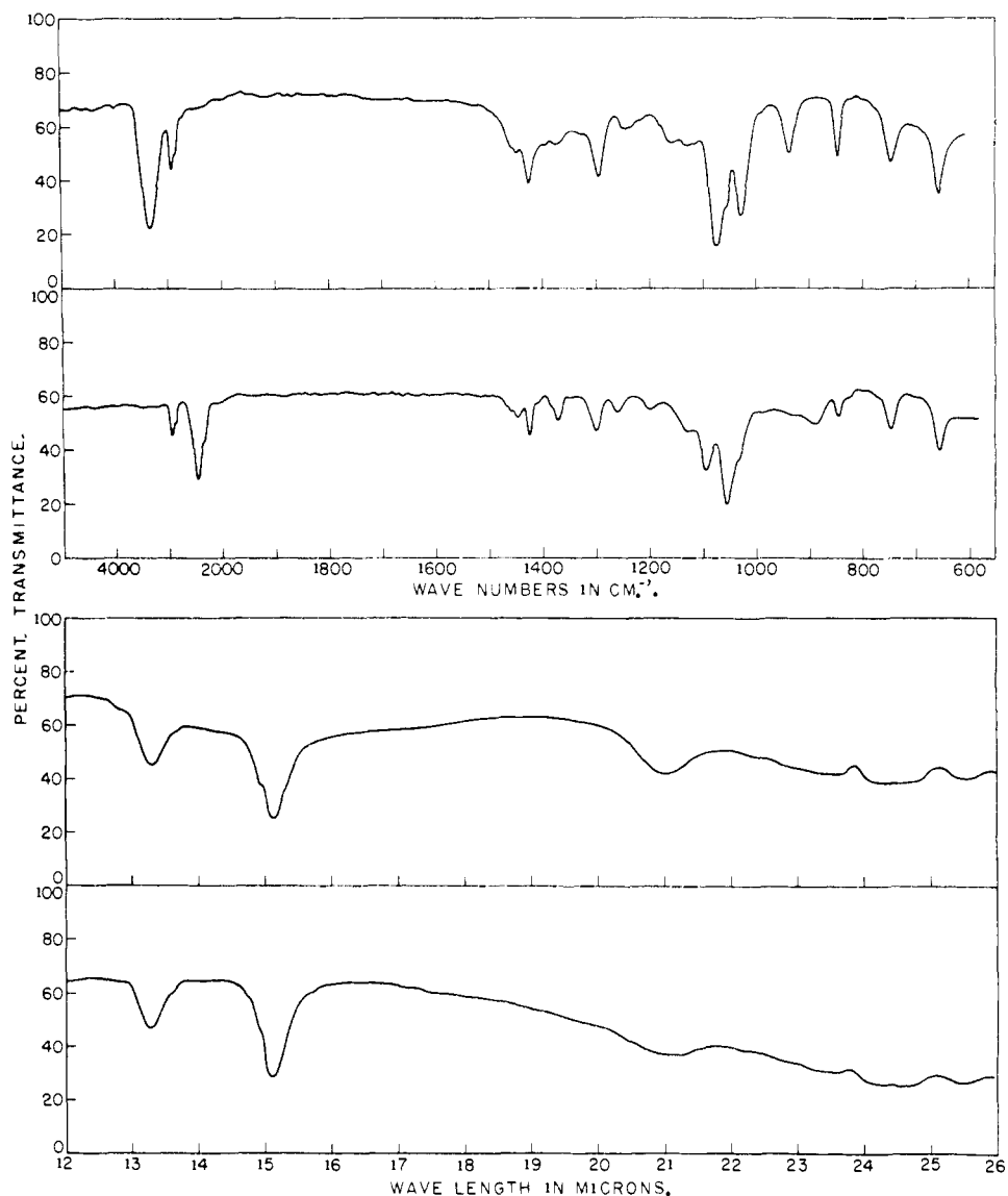
Fig. 1.—Infrared spectra of 2-chloroethanol and 2-chloroethanol- d in the NaCl region (top) and KBr region (bottom).
